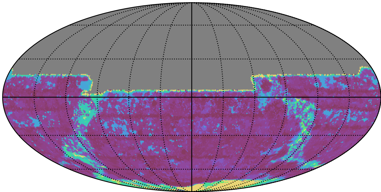
too_elab_r32_d2_griz_v3.4_10yrs All sky y band: Max Inter-Night Gap
