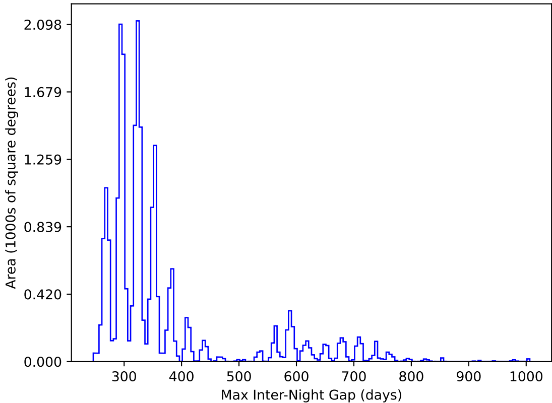
too_elab_r32_d2_griz_v3.4_10yrs All sky y band: Max Inter-Night Gap
