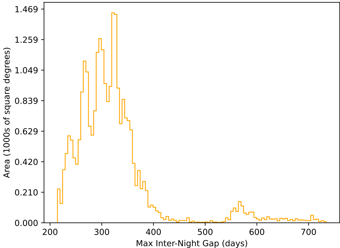
too_elab_r32_d2_griz_v3.4_10yrs All sky r band: Max Inter-Night Gap
