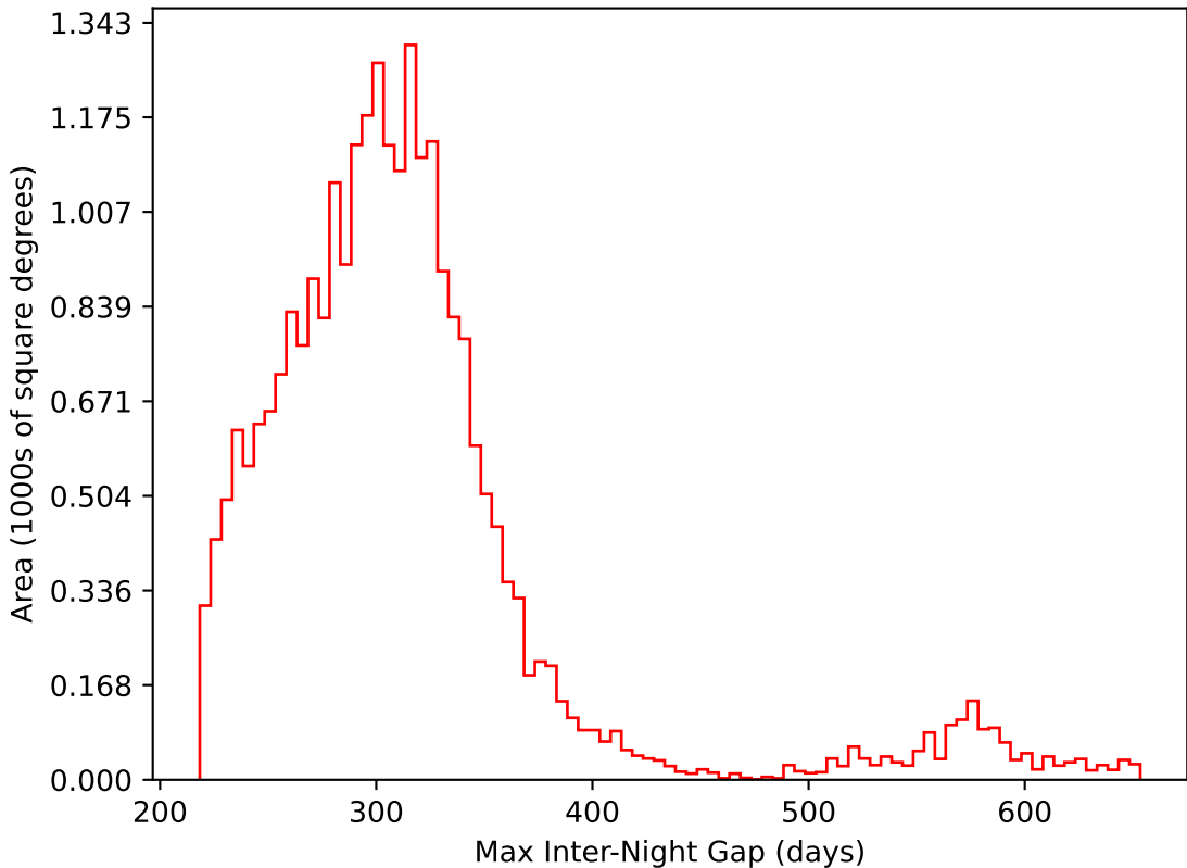
too_elab_r32_d2_griz_v3.4_10yrs All sky i band: Max Inter-Night Gap
