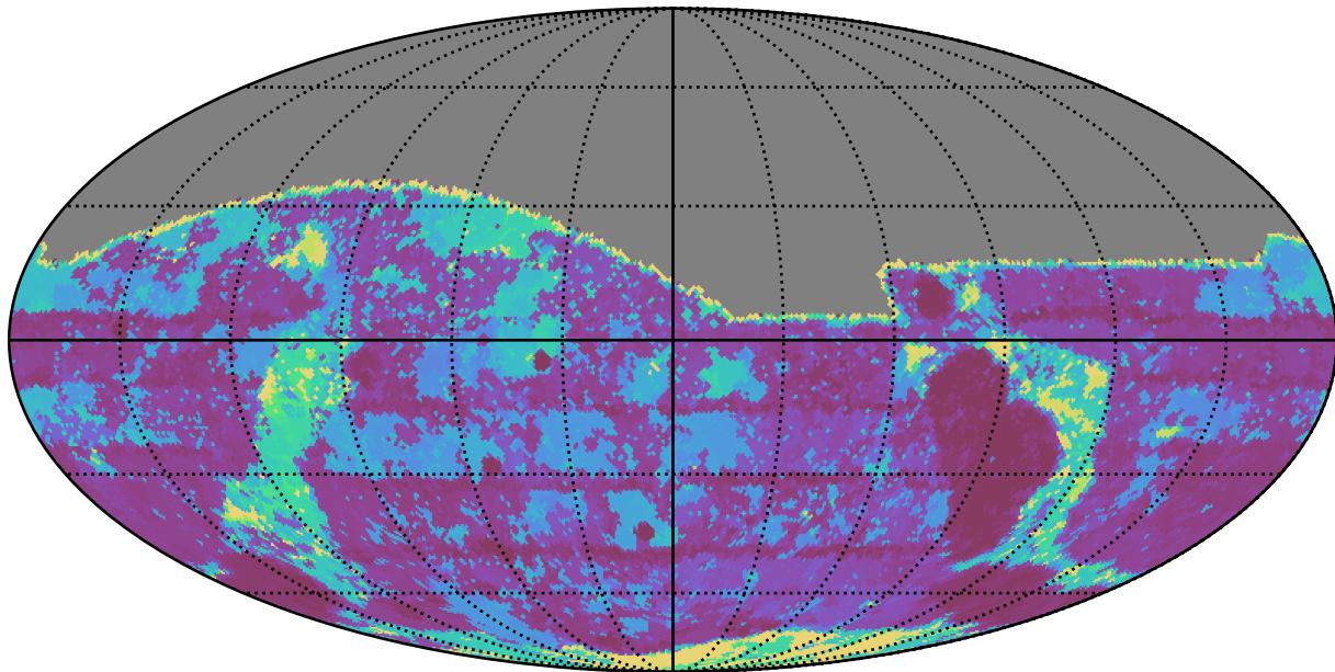
too_elab_r32_d2_griz_v3.4_10yrs All sky g band: Max Inter-Night Gap
