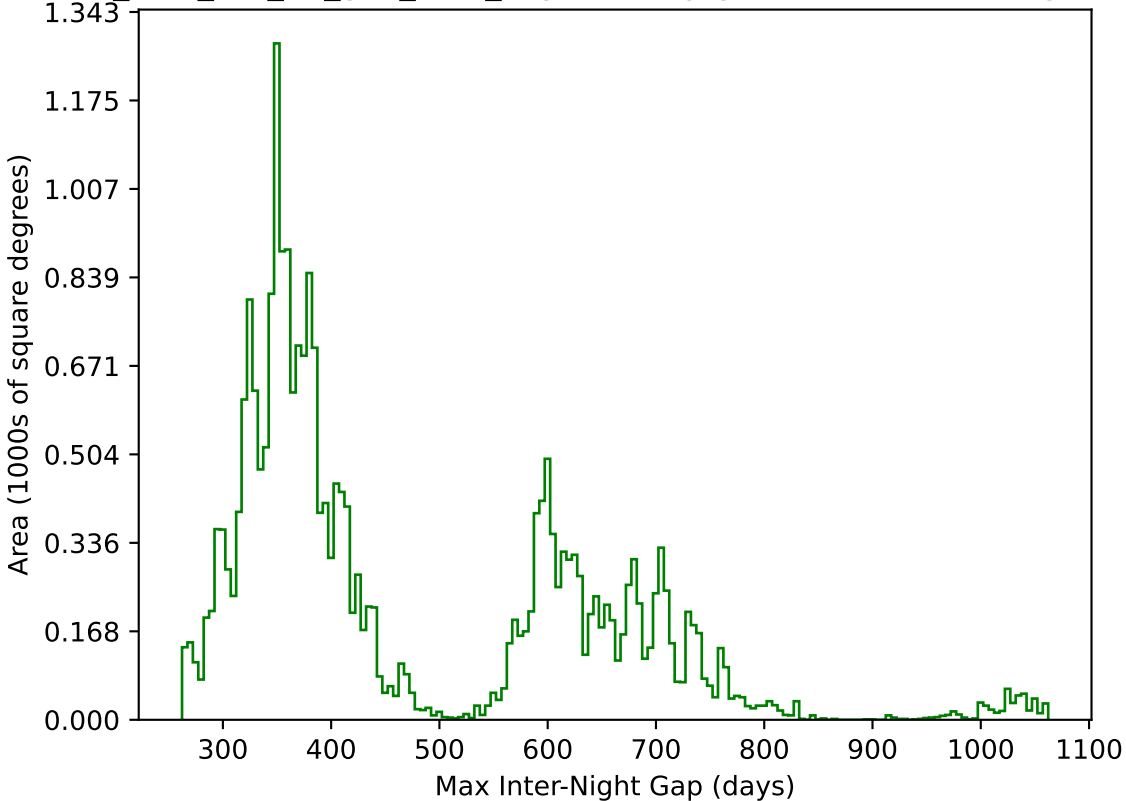
too_elab_r32_d2_griz_v3.4_10yrs All sky g band: Max Inter-Night Gap
