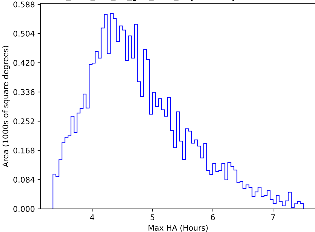
too_elab_r32_d2_griz_v3.4_10yrs WFD y band: Max HA
