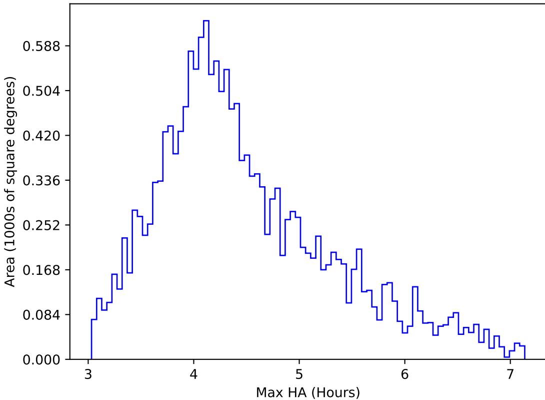
too_elab_r32_d2_griz_v3.4_10yrs WFD r band: Max HA
