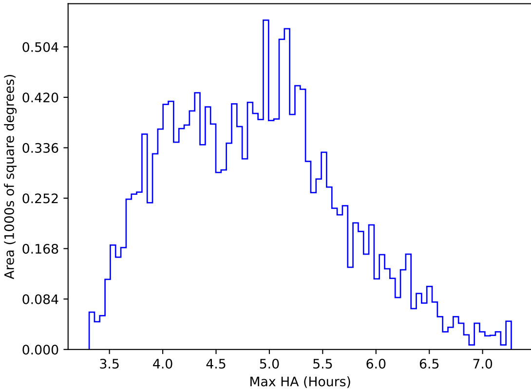
too_elab_r32_d2_griz_v3.4_10yrs WFD i band: Max HA
