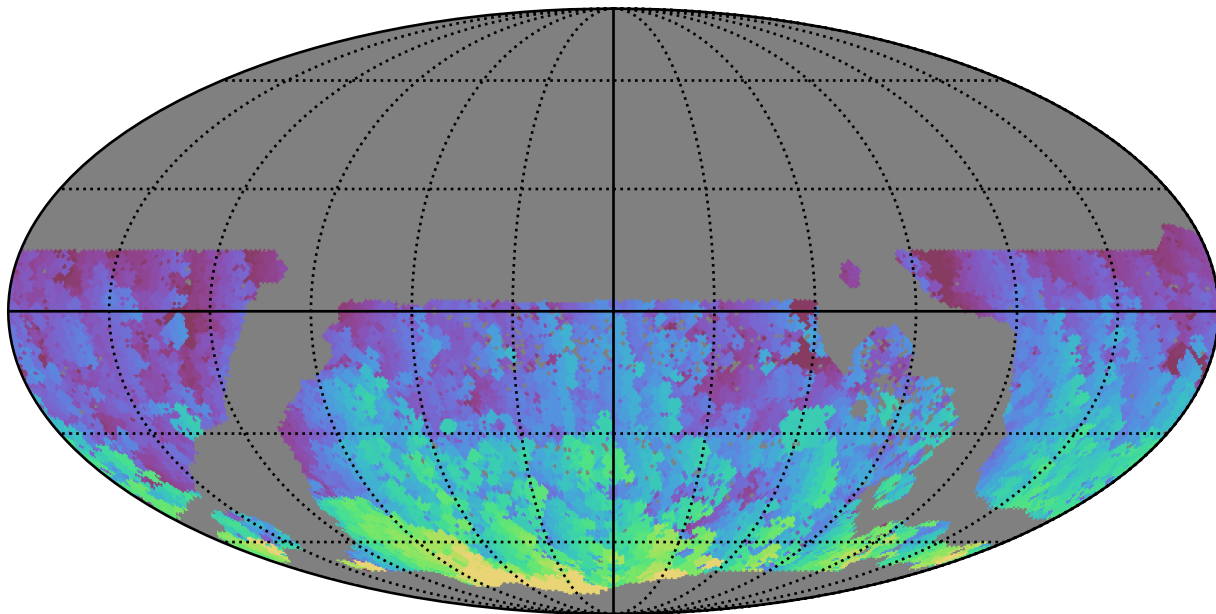
too_elab_r32_d2_griz_v3.4_10yrs WFD g band: Max HA
