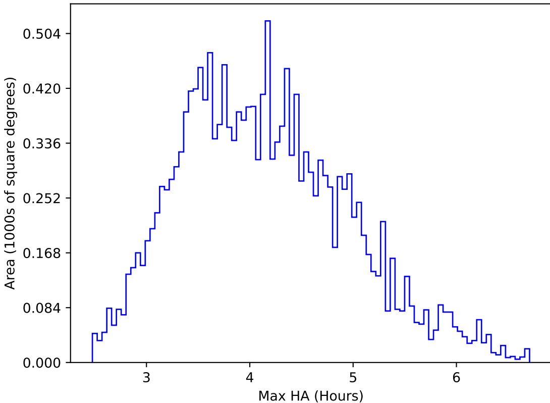
too_elab_r32_d2_griz_v3.4_10yrs WFD g band: Max HA
