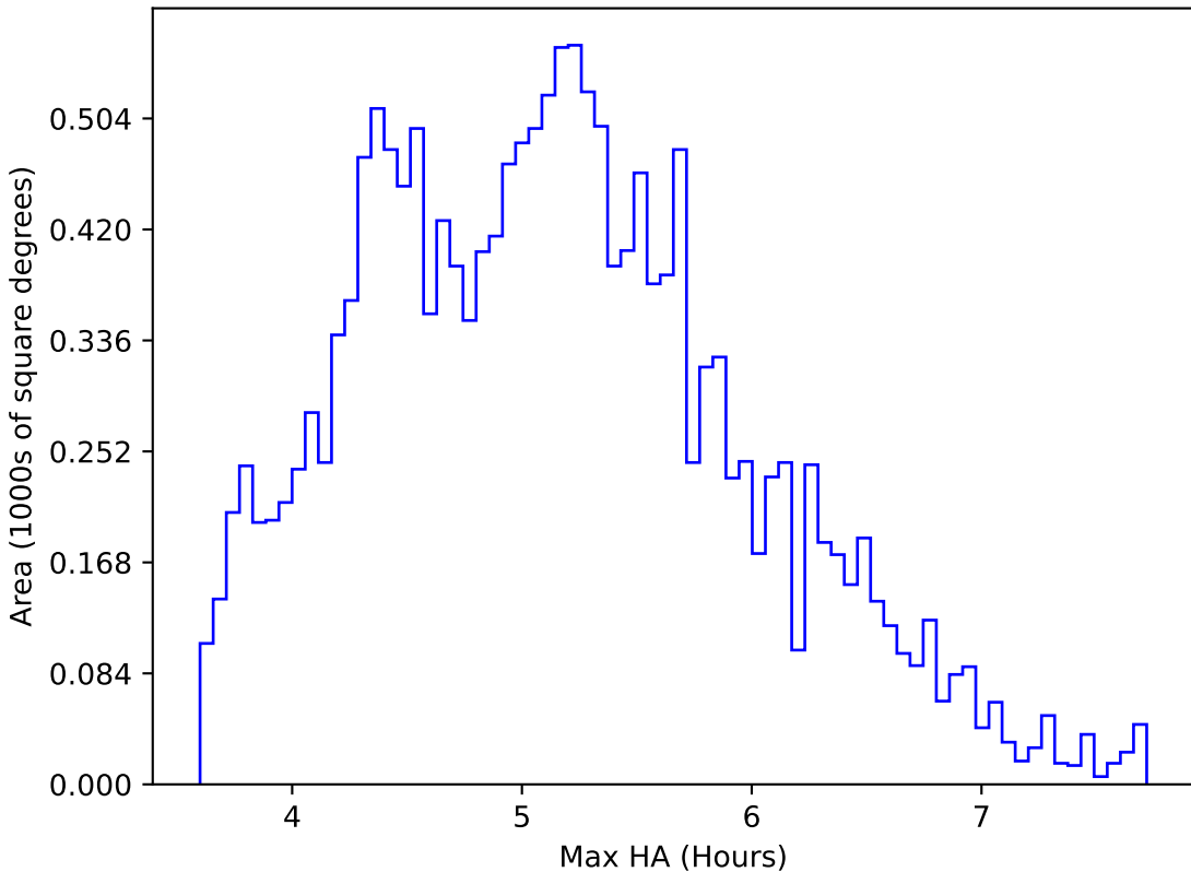
too_elab_r32_d2_griz_v3.4_10yrs WFD all bands: Max HA
