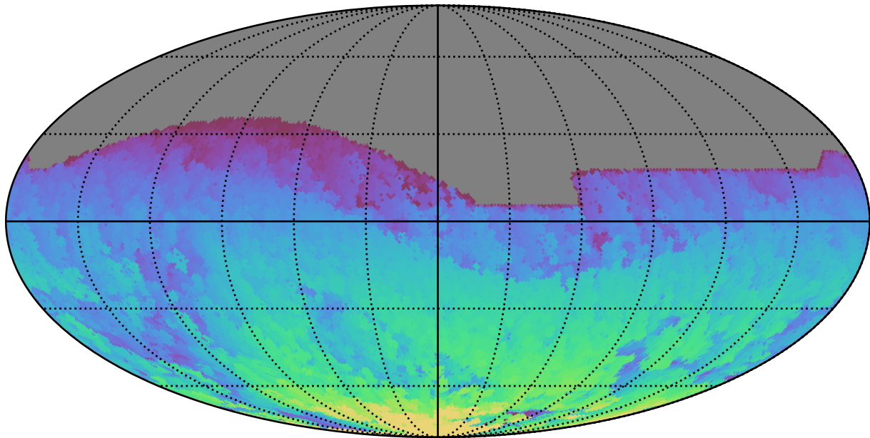
too_elab_r32_d2_griz_v3.4_10yrs All sky z band: Max HA
