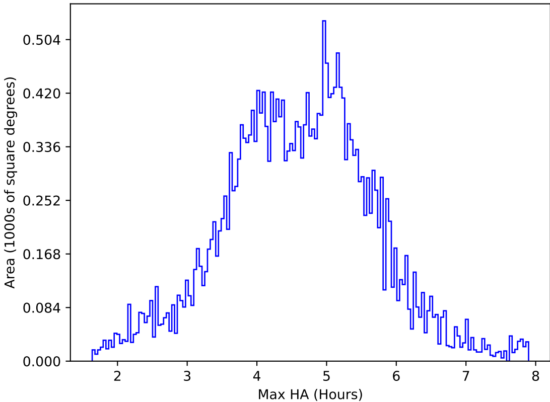
too_elab_r32_d2_griz_v3.4_10yrs All sky z band: Max HA
