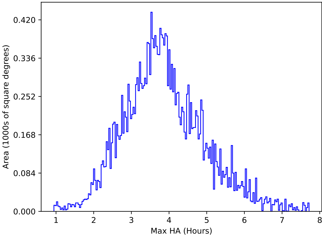
too_elab_r32_d2_griz_v3.4_10yrs All sky u band: Max HA
