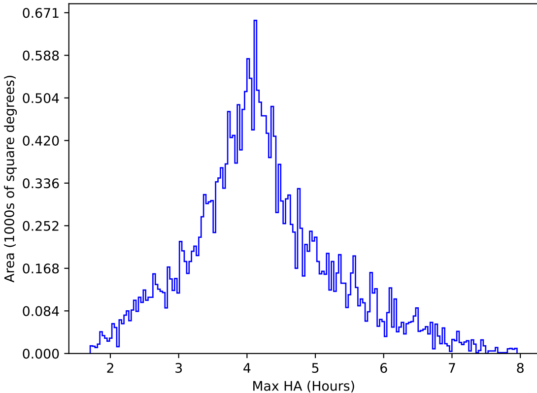
too_elab_r32_d2_griz_v3.4_10yrs All sky r band: Max HA
