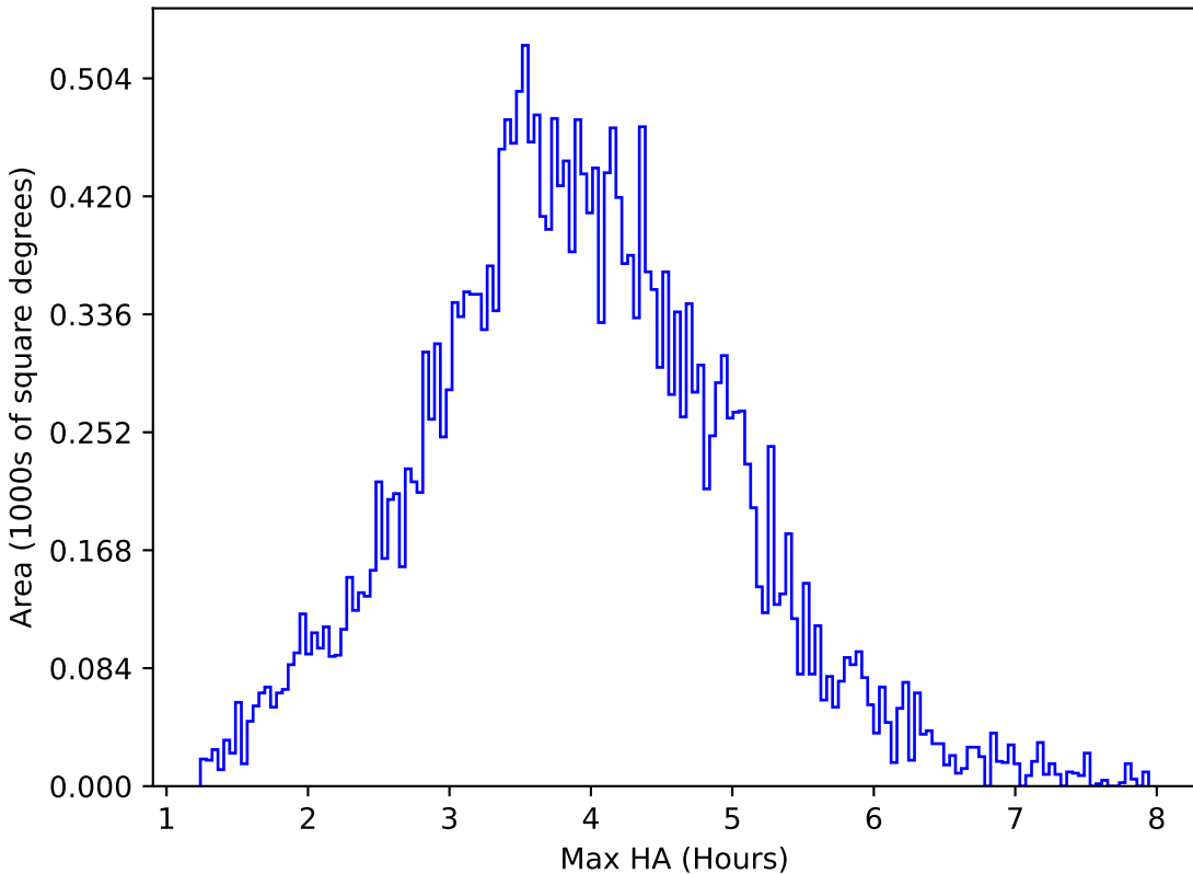
too_elab_r32_d2_griz_v3.4_10yrs All sky g band: Max HA
