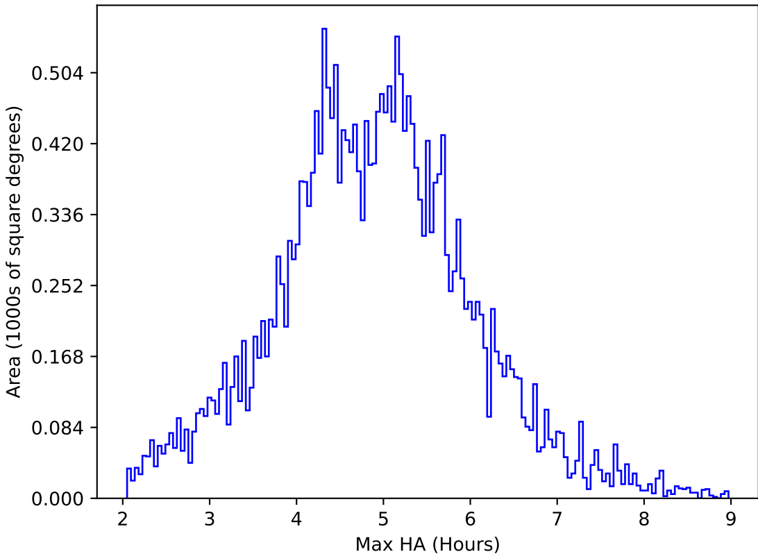
too_elab_r32_d2_griz_v3.4_10yrs All sky all bands: Max HA
