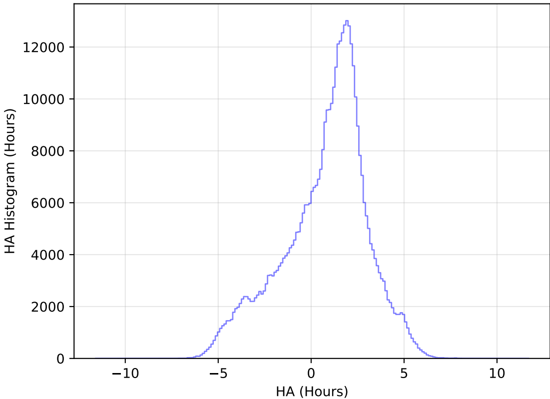
too_elab_r32_d2_griz_v3.4_10yrs WFD z band: HA Histogram
