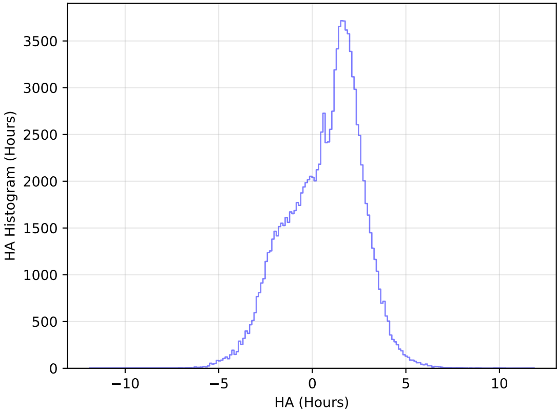
too_elab_r32_d2_griz_v3.4_10yrs WFD u band: HA Histogram
