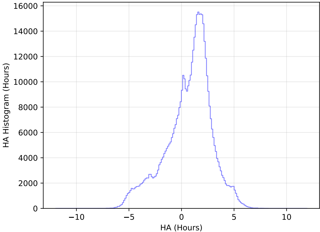
too_elab_r32_d2_griz_v3.4_10yrs WFD i band: HA Histogram
