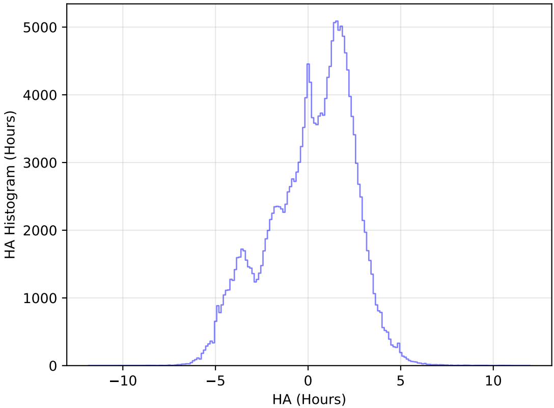
too_elab_r32_d2_griz_v3.4_10yrs WFD g band: HA Histogram
