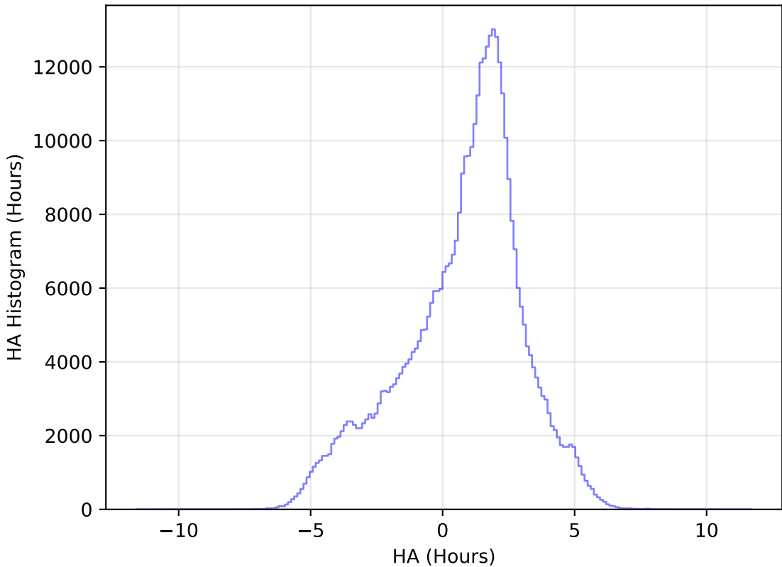
too_elab_r32_d2_griz_v3.4_10yrs All sky z band: HA Histogram
