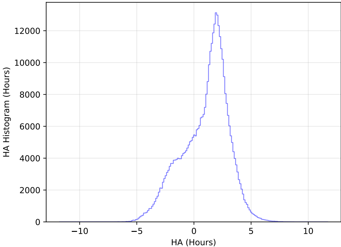
too_elab_r32_d2_griz_v3.4_10yrs All sky y band: HA Histogram
