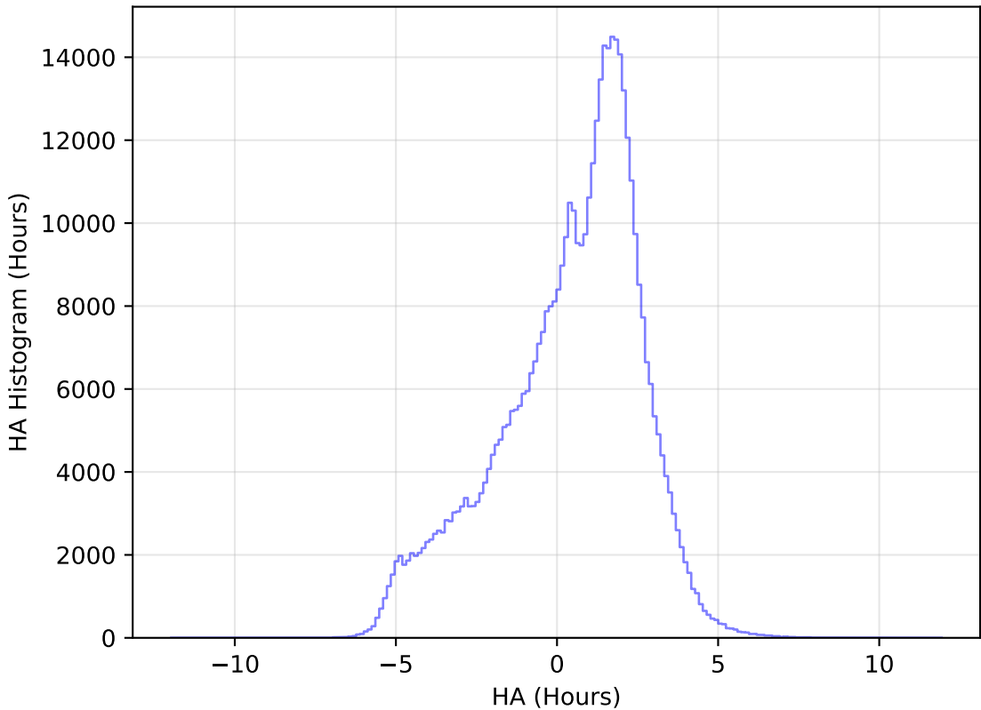
too_elab_r32_d2_griz_v3.4_10yrs All sky r band: HA Histogram
