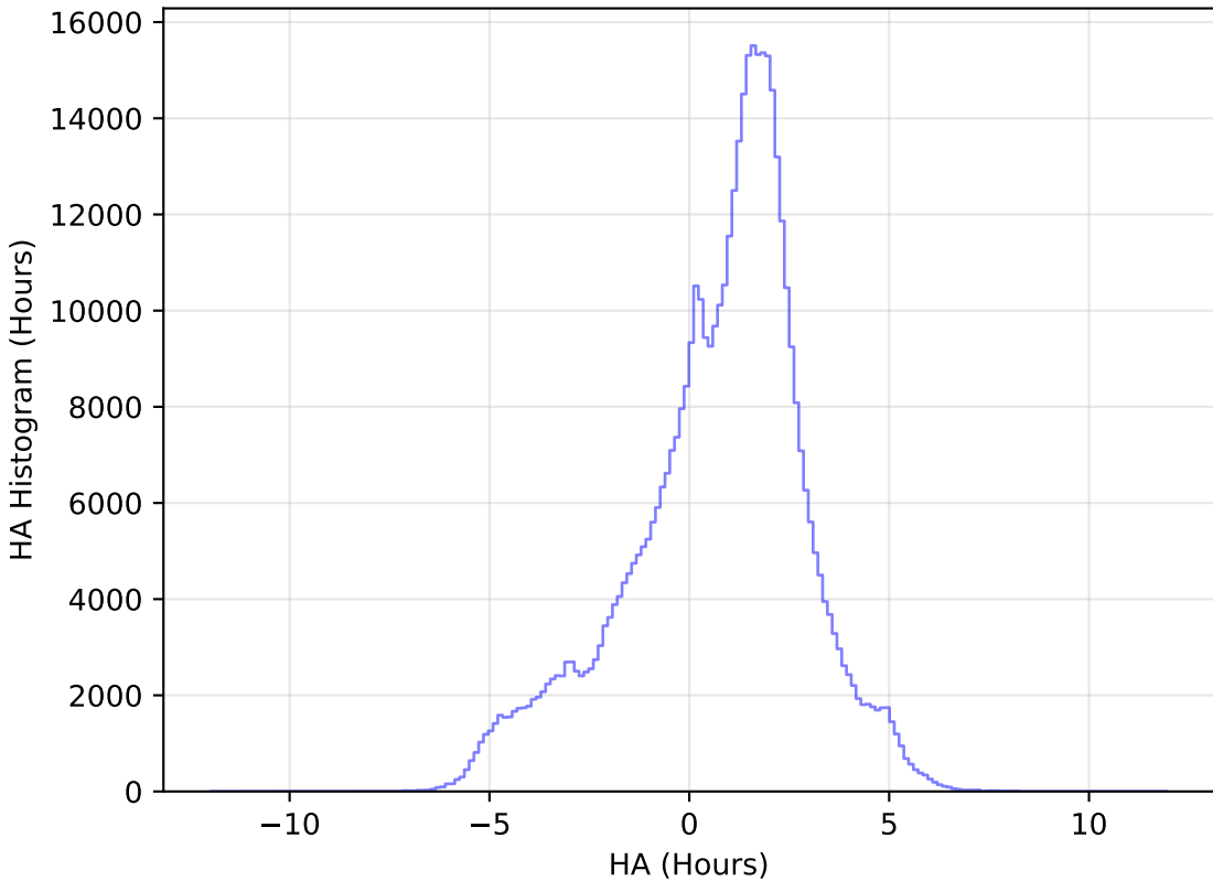
too_elab_r32_d2_griz_v3.4_10yrs All sky i band: HA Histogram
