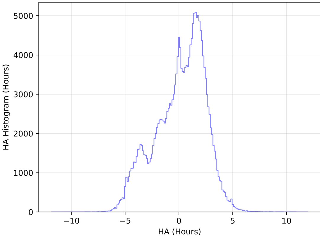
too_elab_r32_d2_griz_v3.4_10yrs All sky g band: HA Histogram
