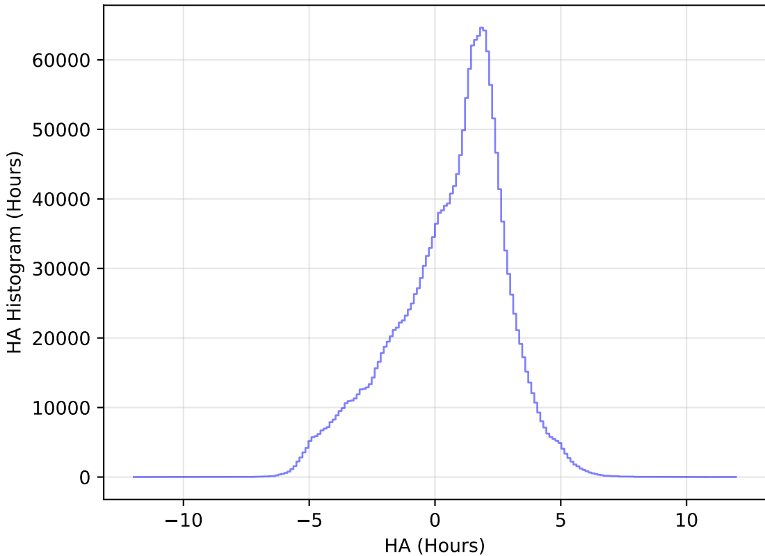
too_elab_r32_d2_griz_v3.4_10yrs All sky all bands: HA Histogram
