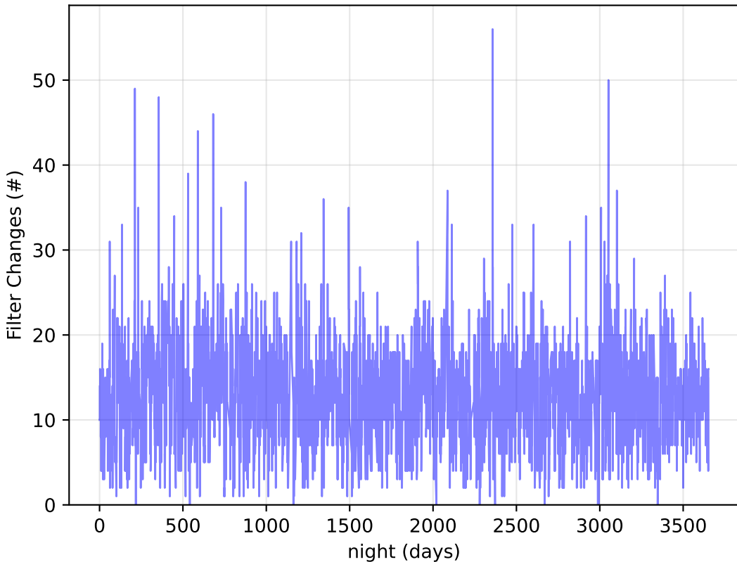
too_elab_r32_d2_griz_v3.4_10yrs Per Night: Filter Changes
