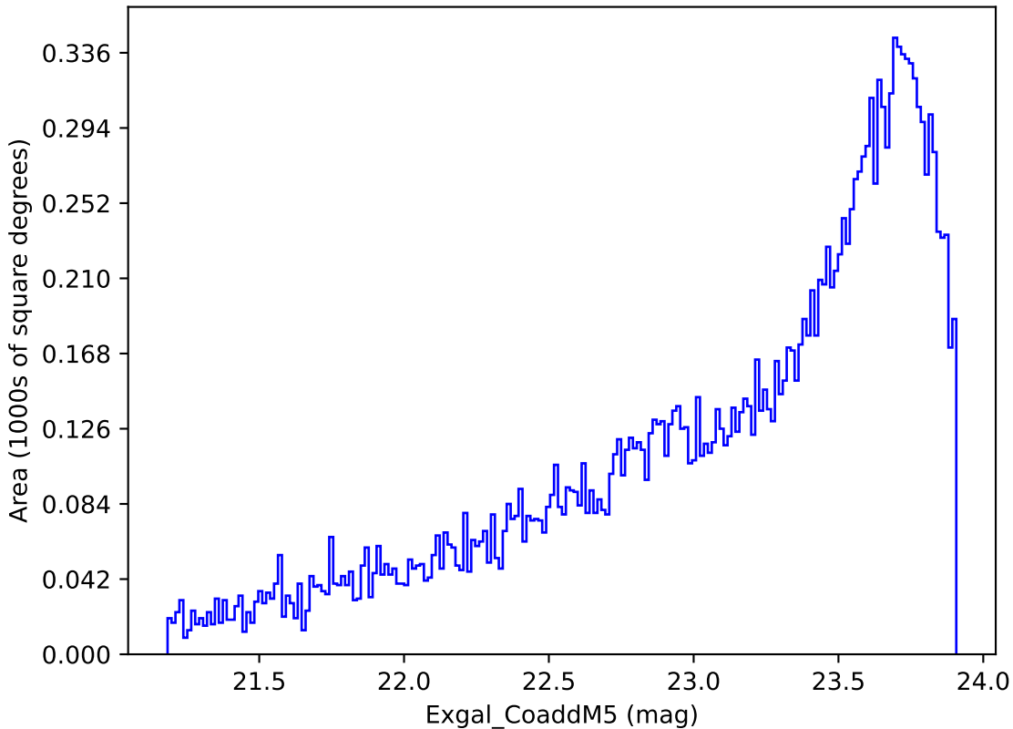
too_elab_r32_d2_griz_v3.4_10yrs Yr 3-4 y band: Exgal_CoaddM5
