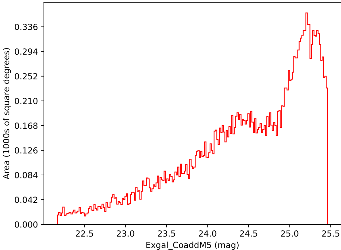
too_elab_r32_d2_griz_v3.4_10yrs Yr 3-4 i band: Exgal_CoaddM5
