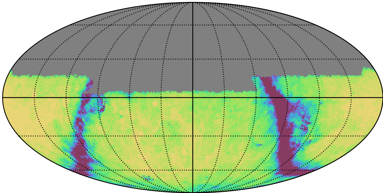
too_elab_r32_d2_griz_v3.4_10yrs Yr 1 u band: Exgal_CoaddM5
