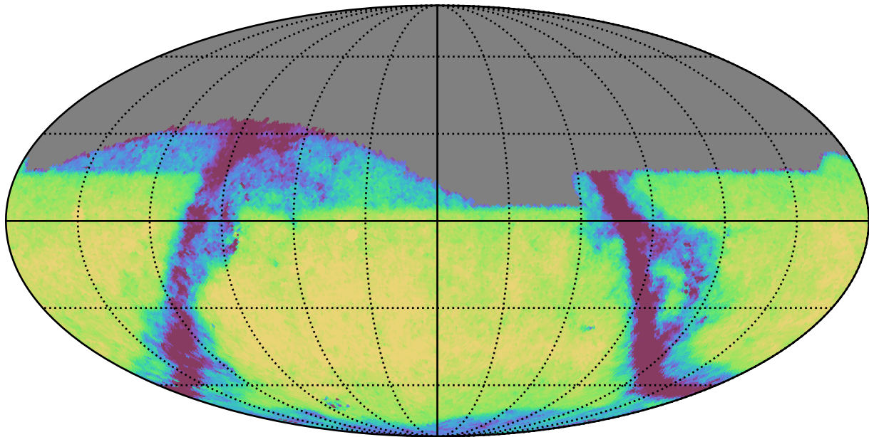
too_elab_r32_d2_griz_v3.4_10yrs Yr 1 i band: Exgal_CoaddM5
