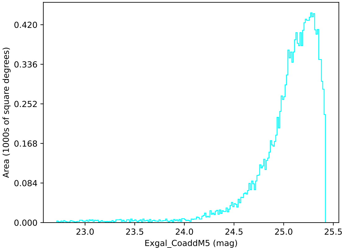
too_elab_r32_d2_griz_v3.4_10yrs WFD u band: Exgal_CoaddM5
