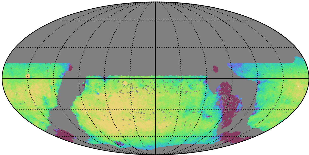
too_elab_r32_d2_griz_v3.4_10yrs WFD i band: Exgal_CoaddM5
