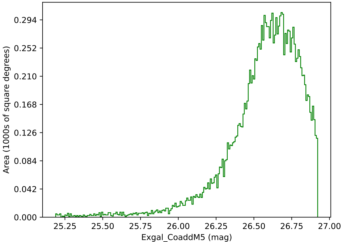
too_elab_r32_d2_griz_v3.4_10yrs WFD g band: Exgal_CoaddM5
