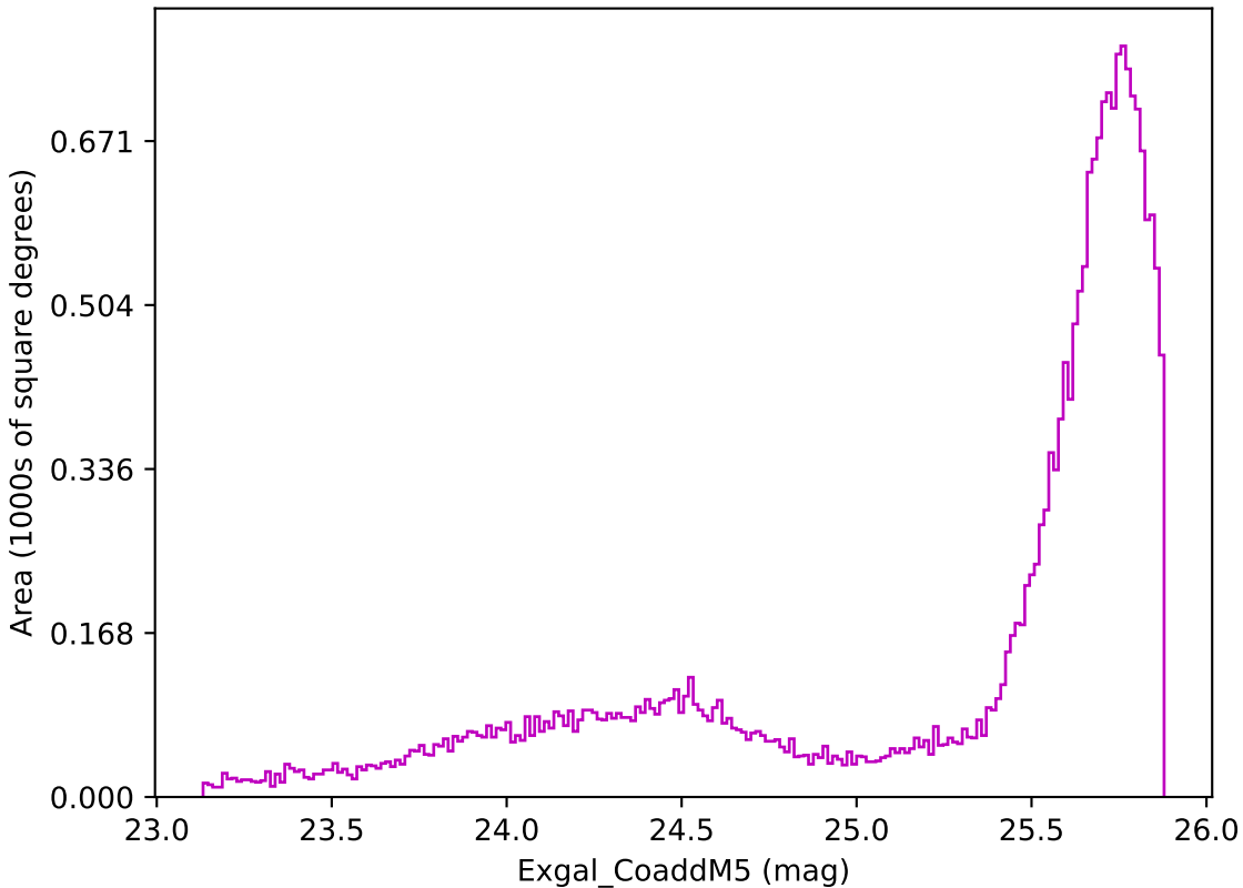
too_elab_r32_d2_griz_v3.4_10yrs All sky z band: Exgal_CoaddM5
