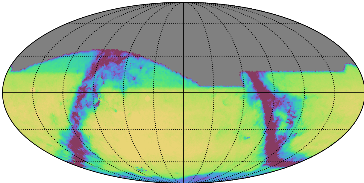
too_elab_r32_d2_griz_v3.4_10yrs All sky r band: Exgal_CoaddM5
