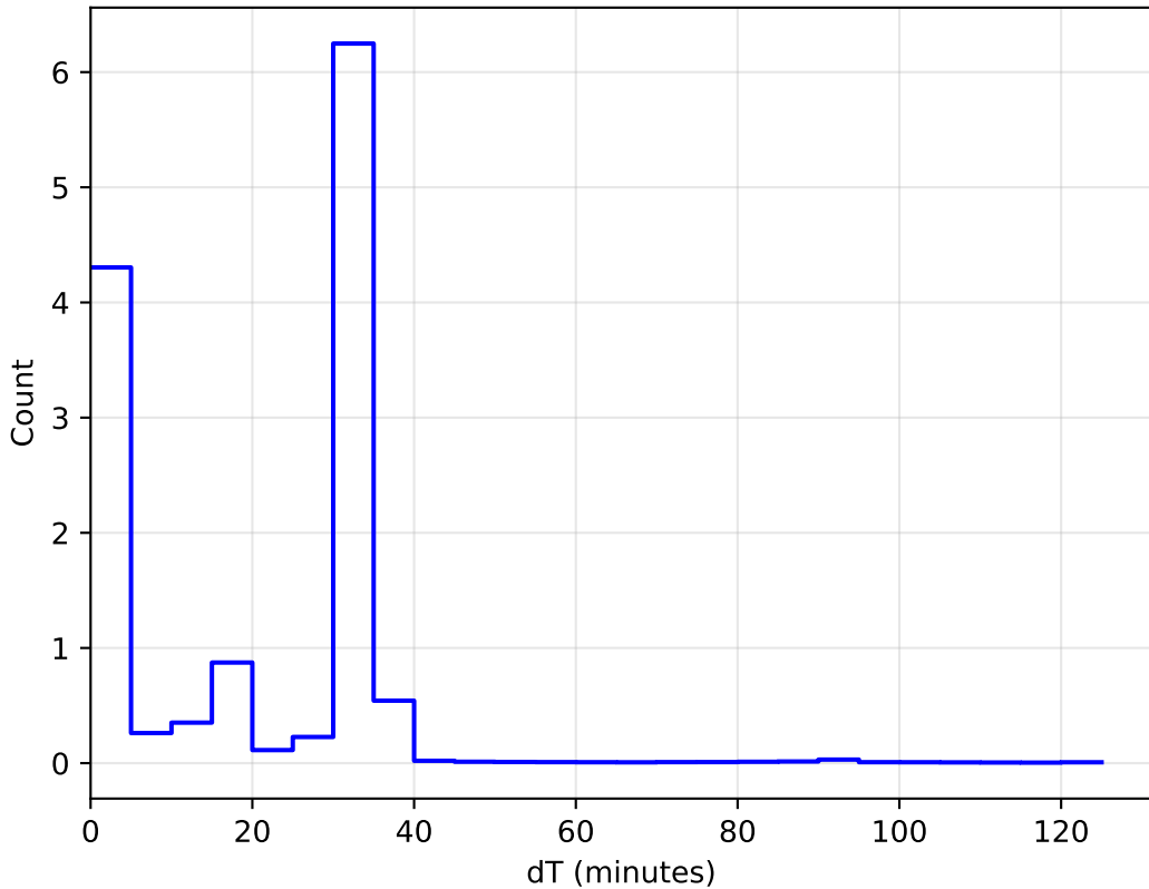
too_elab_r32_d2_griz_v3.4_10yrs All sky: DeltaT Histogram 1e6
