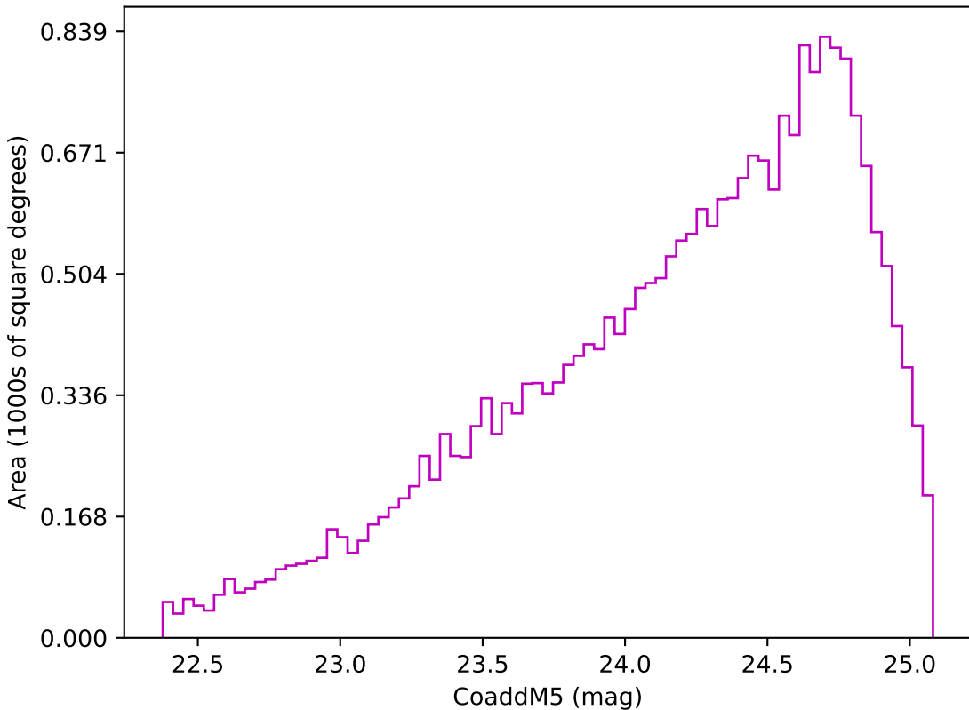
too_elab_r32_d2_griz_v3.4_10yrs Yr 3-4 z band: CoaddM5
