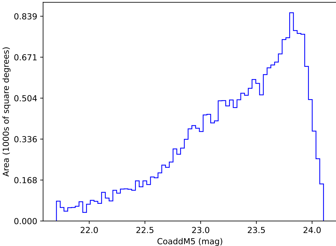
too_elab_r32_d2_griz_v3.4_10yrs Yr 3-4 y band: CoaddM5
