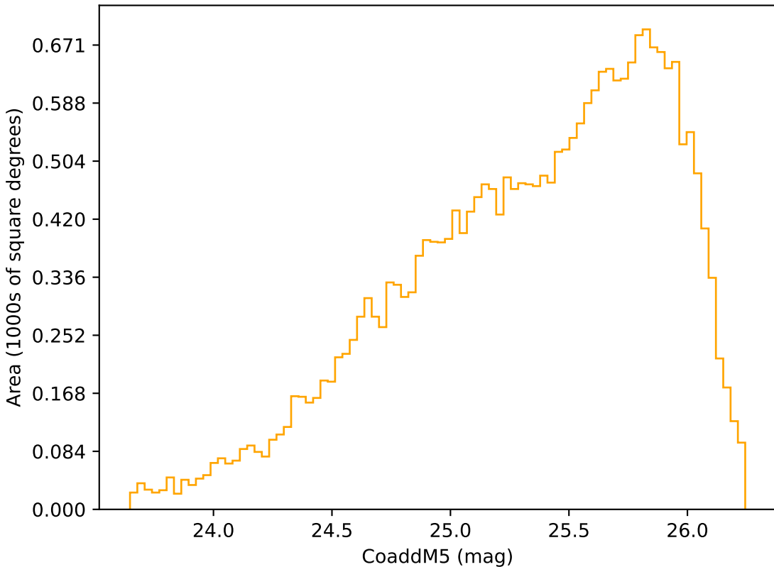
too_elab_r32_d2_griz_v3.4_10yrs Yr 3-4 r band: CoaddM5
