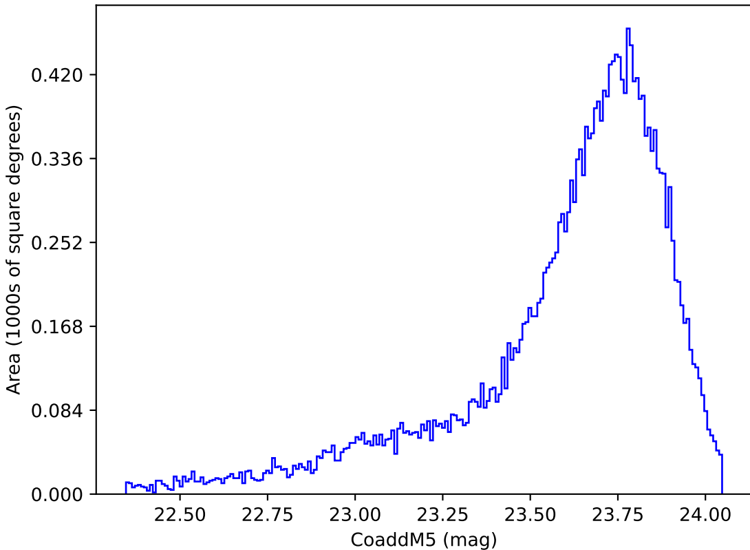
too_elab_r32_d2_griz_v3.4_10yrs Yr 1 y band: CoaddM5
