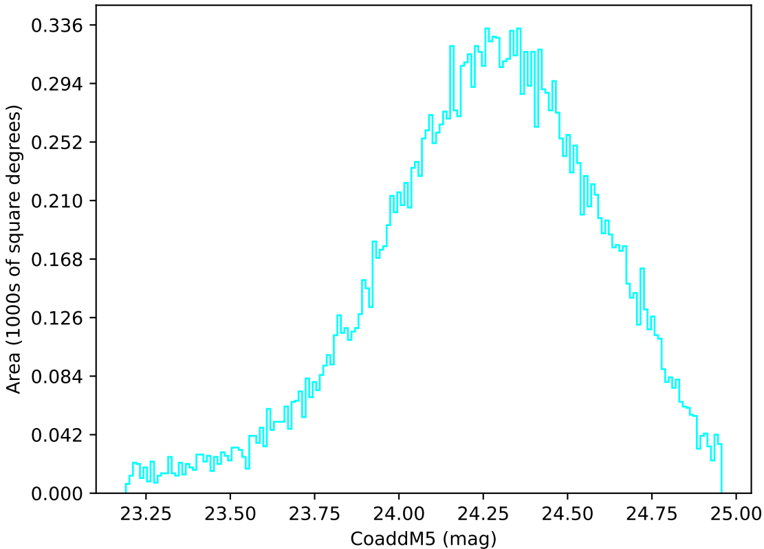
too_elab_r32_d2_griz_v3.4_10yrs Yr 1 u band: CoaddM5
