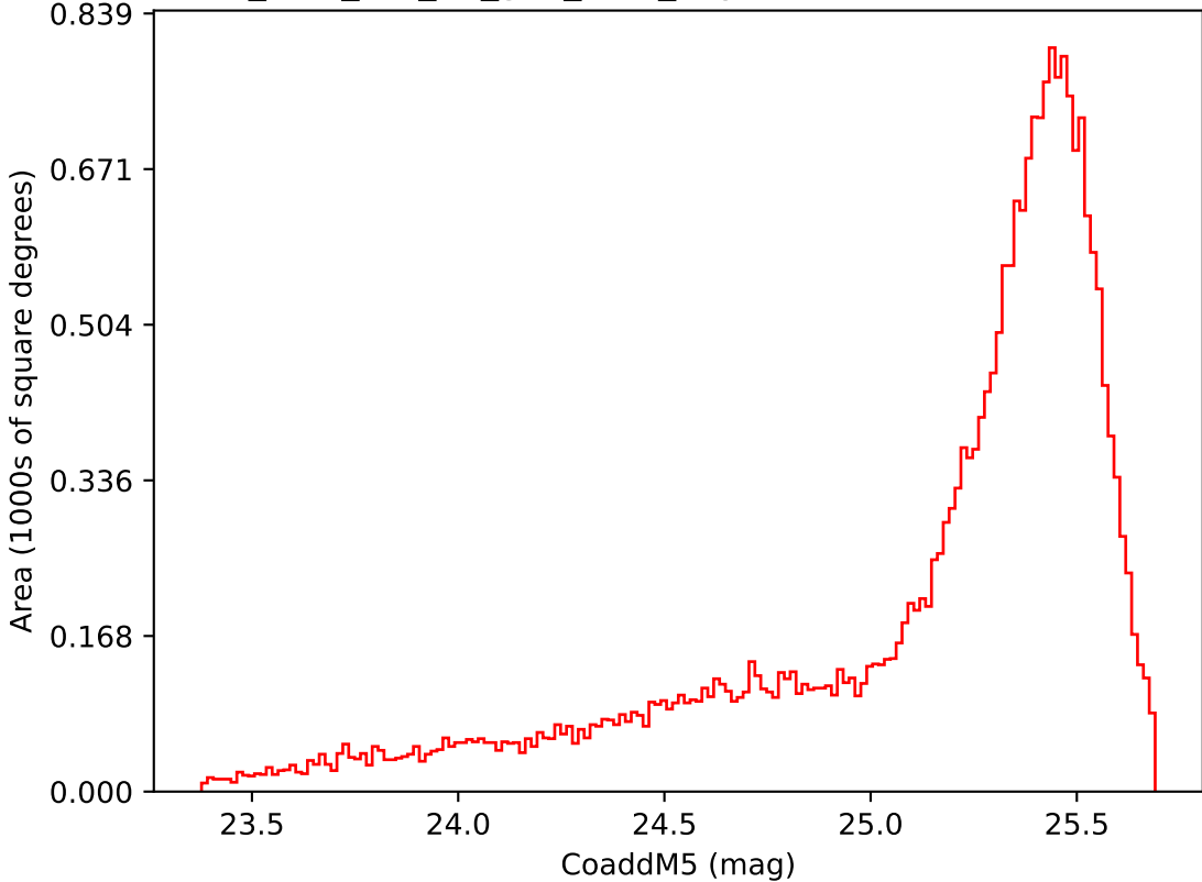
too_elab_r32_d2_griz_v3.4_10yrs Yr 1 i band: CoaddM5
