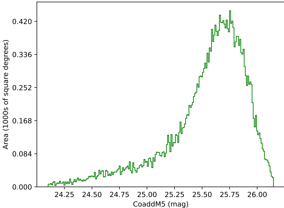
too_elab_r32_d2_griz_v3.4_10yrs Yr 1 g band: CoaddM5
