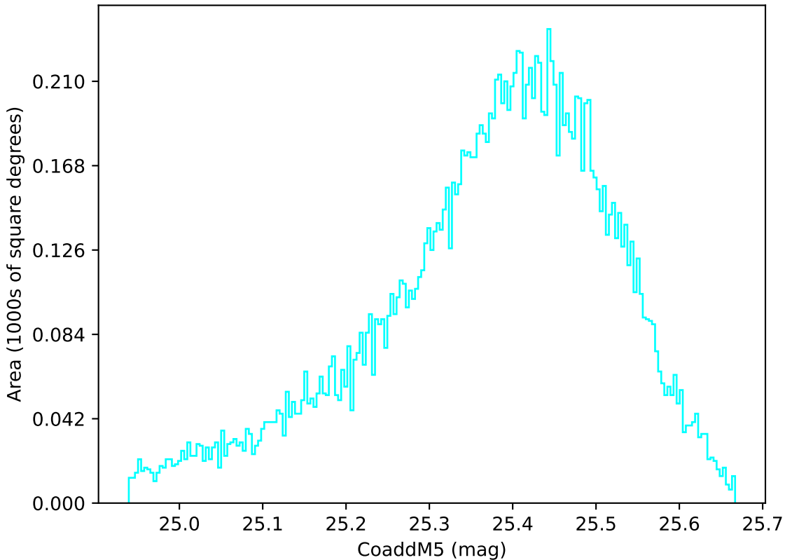
too_elab_r32_d2_griz_v3.4_10yrs WFD u band: CoaddM5
