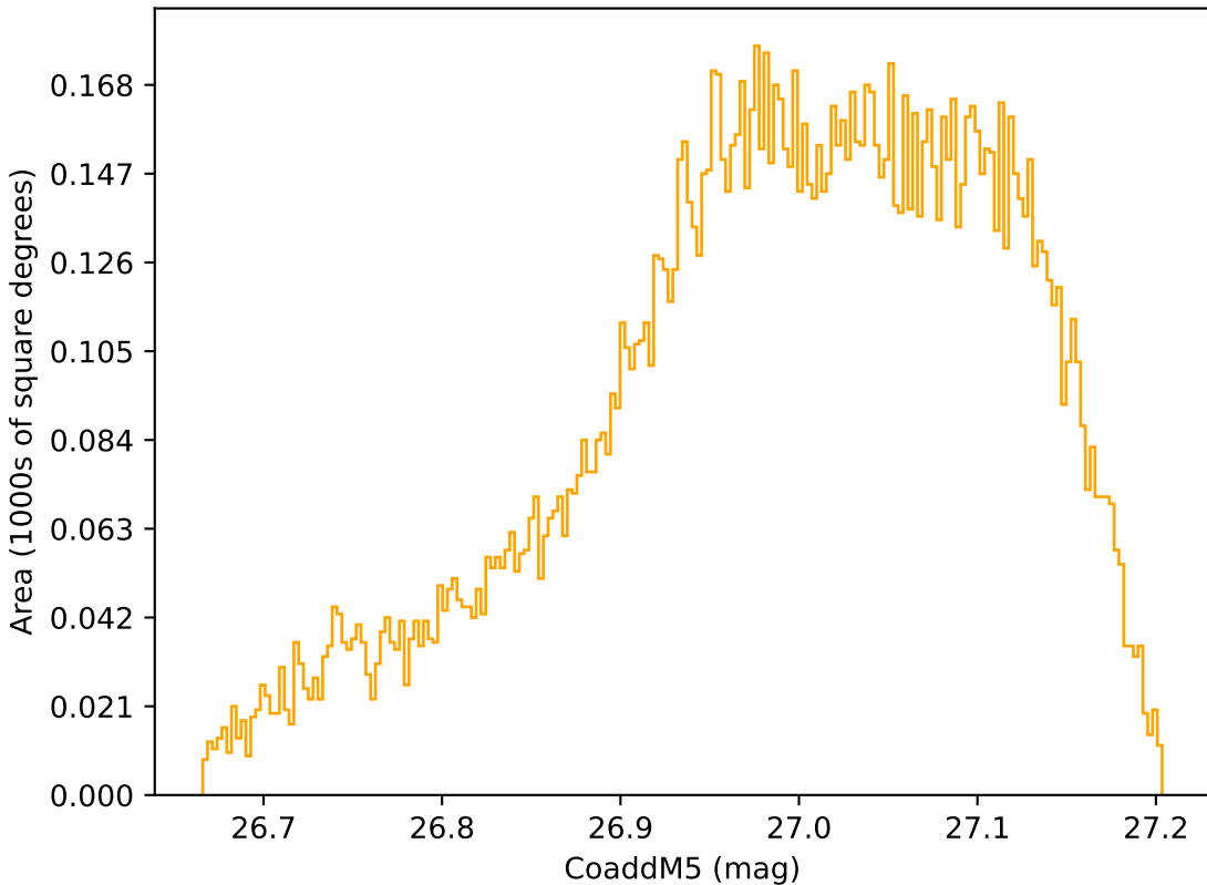
too_elab_r32_d2_griz_v3.4_10yrs WFD r band: CoaddM5
