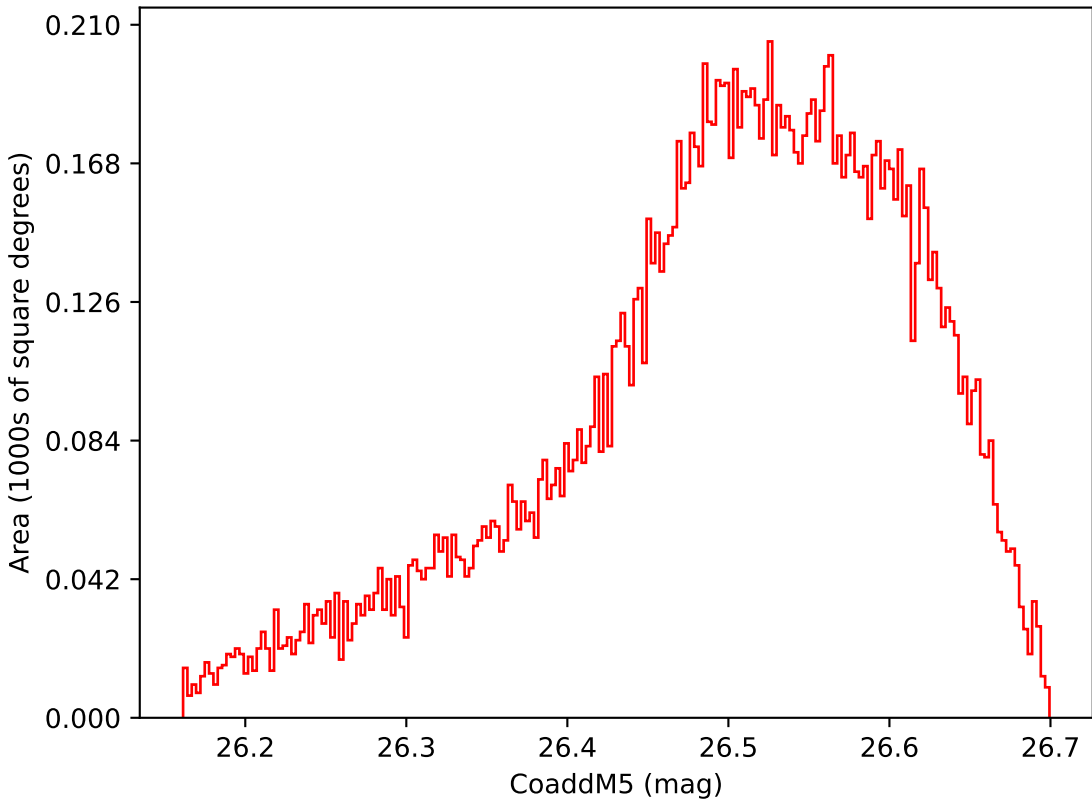
too_elab_r32_d2_griz_v3.4_10yrs WFD i band: CoaddM5
