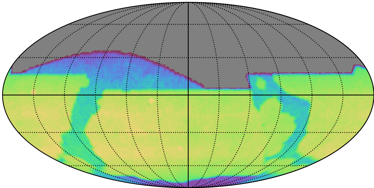
too_elab_r32_d2_griz_v3.4_10yrs All sky z band: CoaddM5
